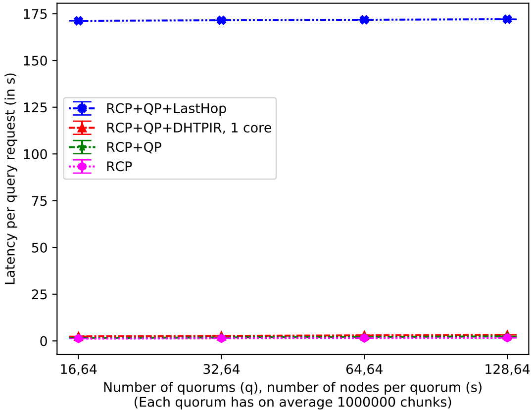
Latency per query vs. number of nodes
