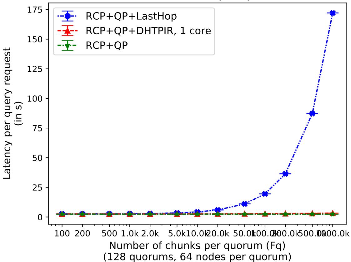
Latency per query vs. number of chunks per quorum
