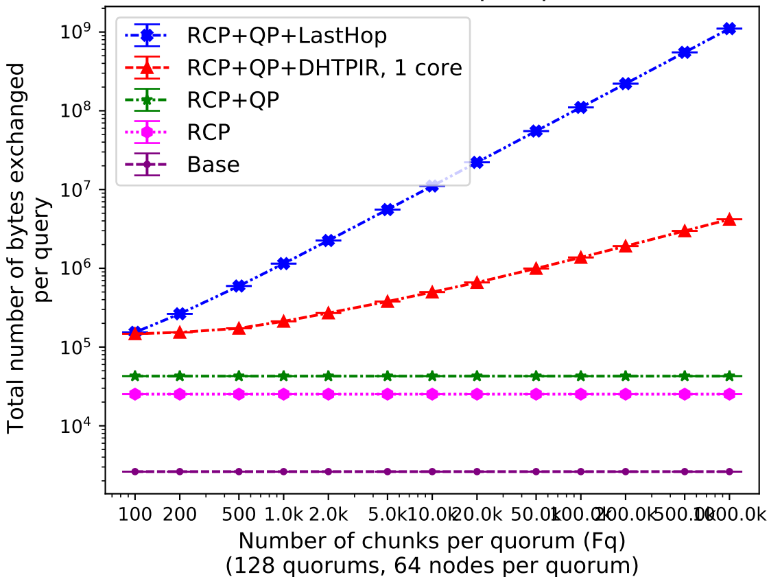
Total communication complexity per query vs. number of chunks per quorum
