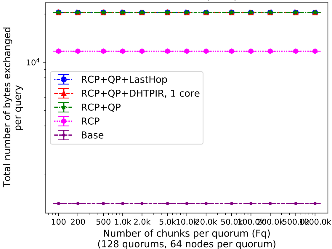
Total publication communication complexity per query vs. number of chunks per quorum
