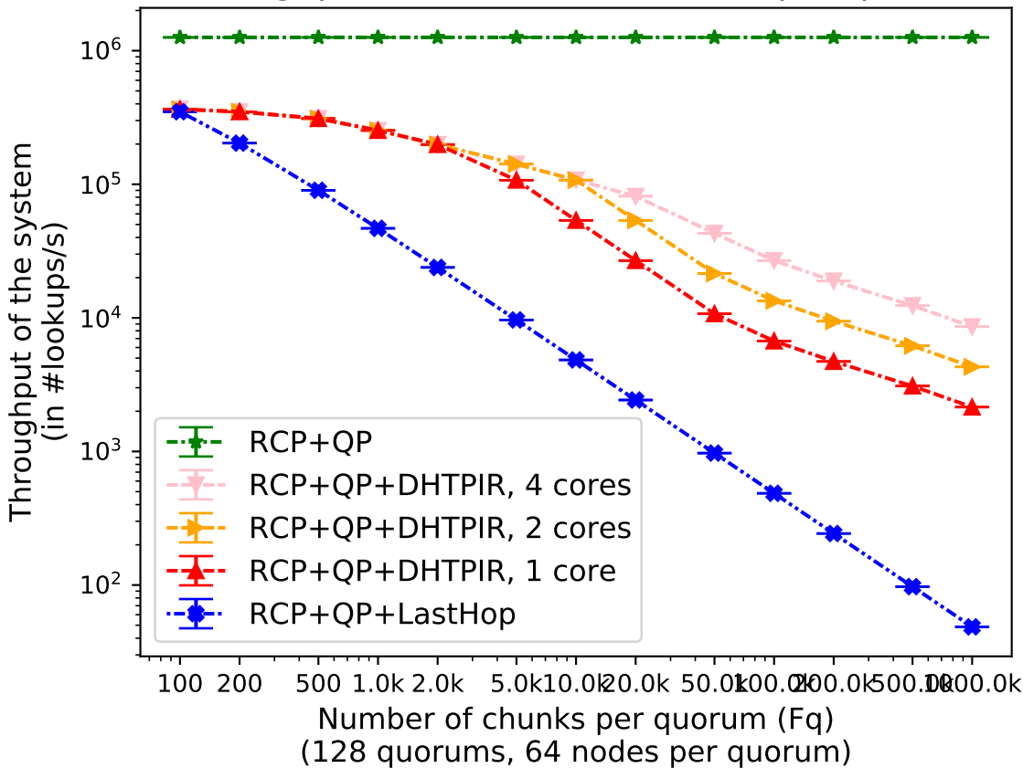
Throughput vs. number of chunks per quorum
