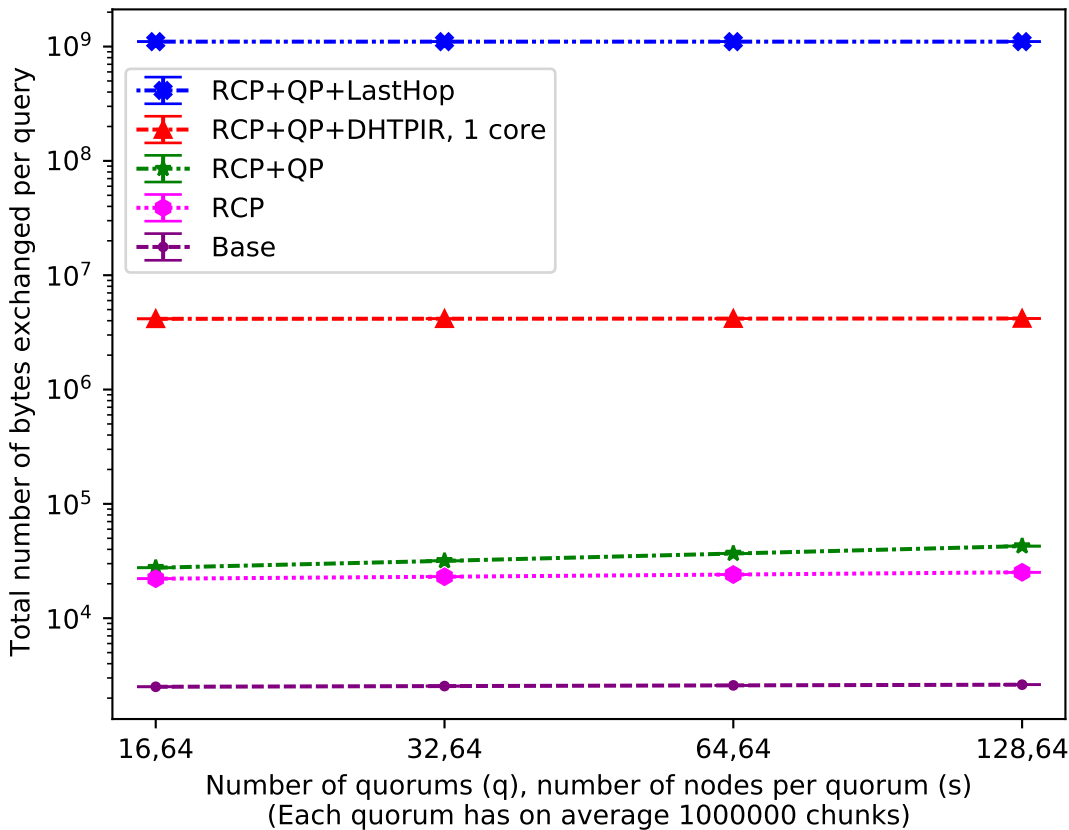
Total communication complexity per query vs. number of nodes
