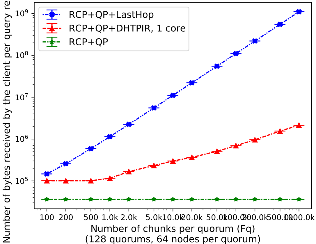
Download communication complexity per query vs. number of chunks per quorum
