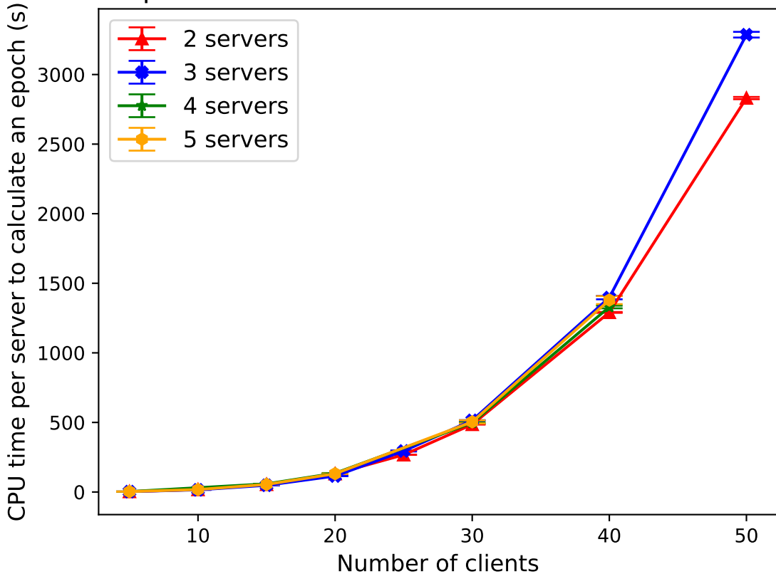
Comparing CPU time for covert security epoch calculations across numbers of servers
