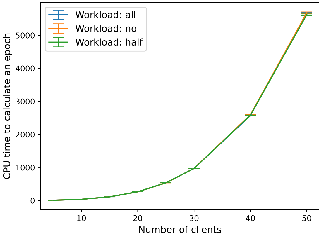
Comparing CPU time for epochs across workloads
