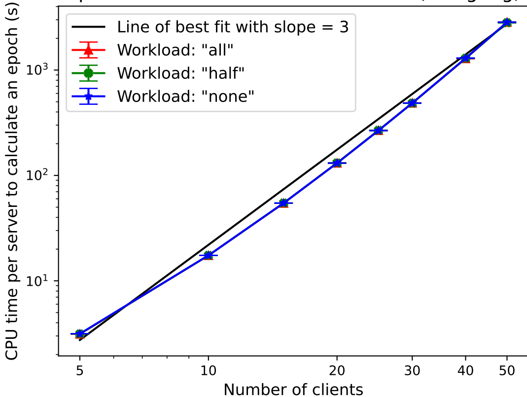
Comparing CPU time for covert security epoch calculations across workloads (in log-log)
