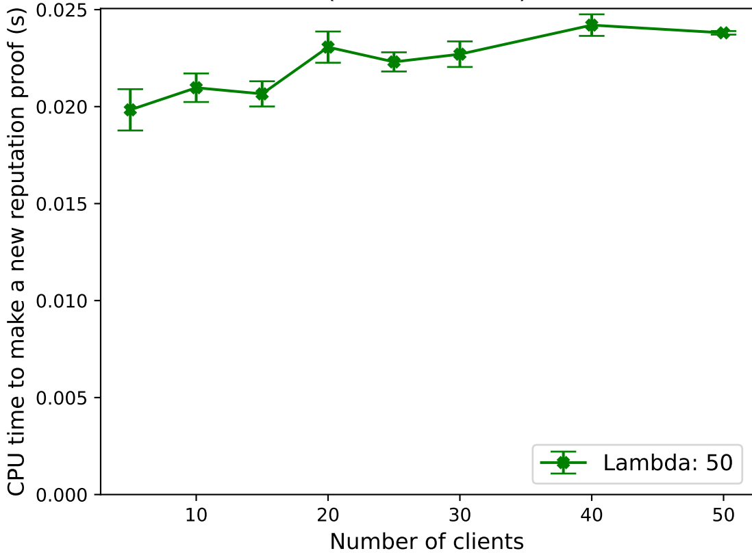
Measuring CPU time for making reputation proofs (in linear scale)
