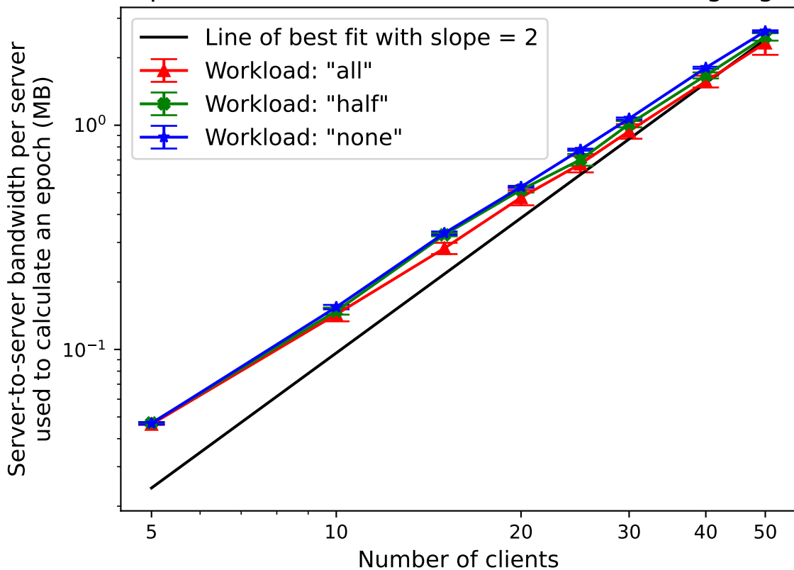
Comparing bandwidth for HbC security epoch calculations across workloads (in log-log)
