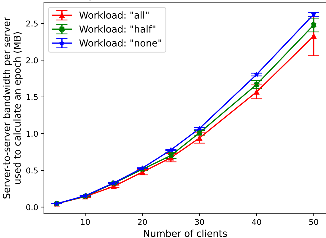
Comparing bandwidth for HbC security epoch calculations across workloads
