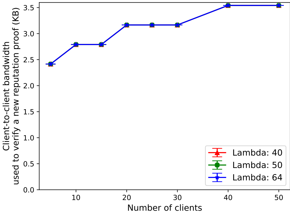
Comparing bandwidth for verifying reputation proofs across different values of lambda
