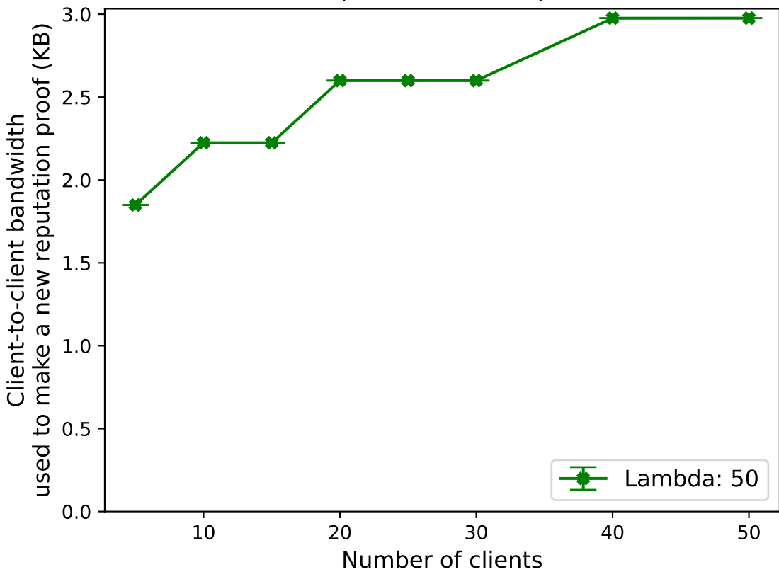
Measuring bandwidth for making reputation proofs (in linear scale)
