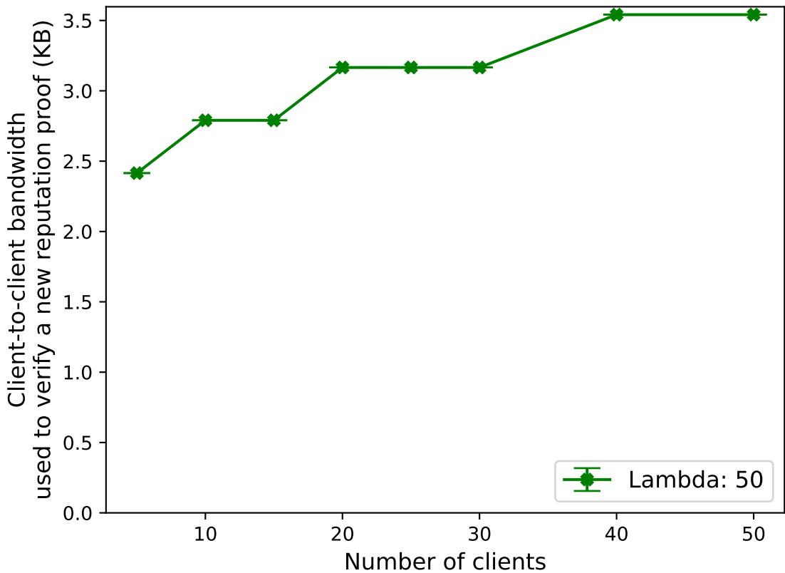
Measuring bandwidth for verifying reputation proofs (in linear scale)
