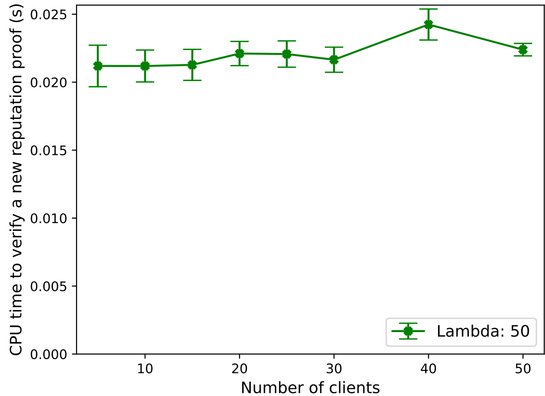
Comparing CPU time for verifying reputation proofs (in linear scale)
