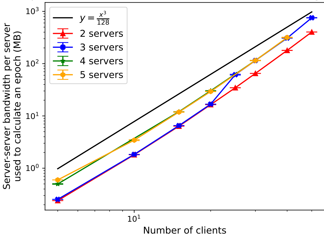
Comparing bandwidth for covert security epoch calculations across numbers of servers (in log-log)
