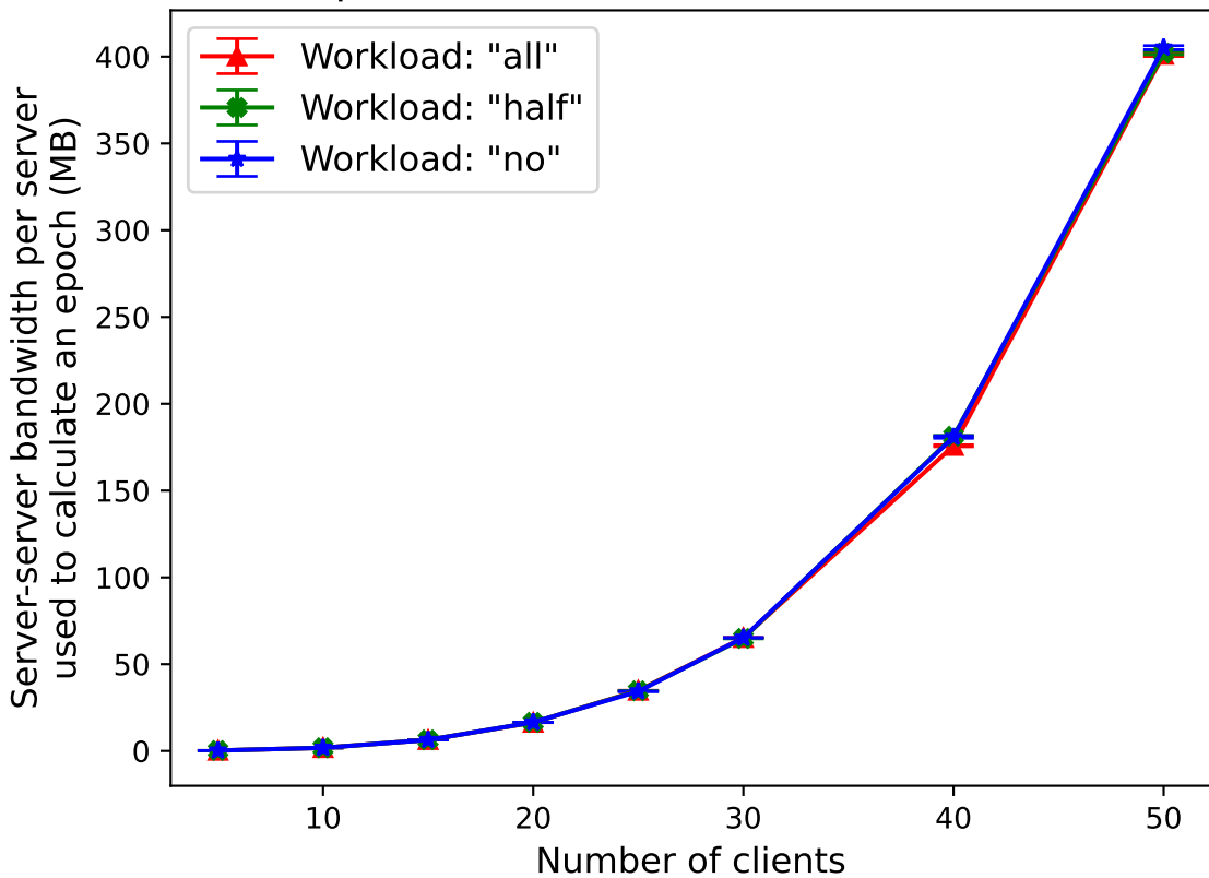
Comparing bandwidth for covert security epoch calculations across workloads
