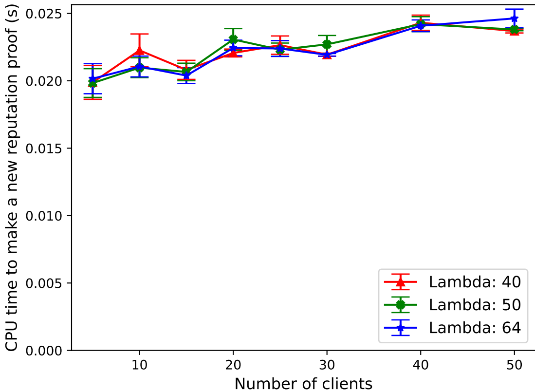
Comparing CPU time for making reputation proofs across different values of lambda
