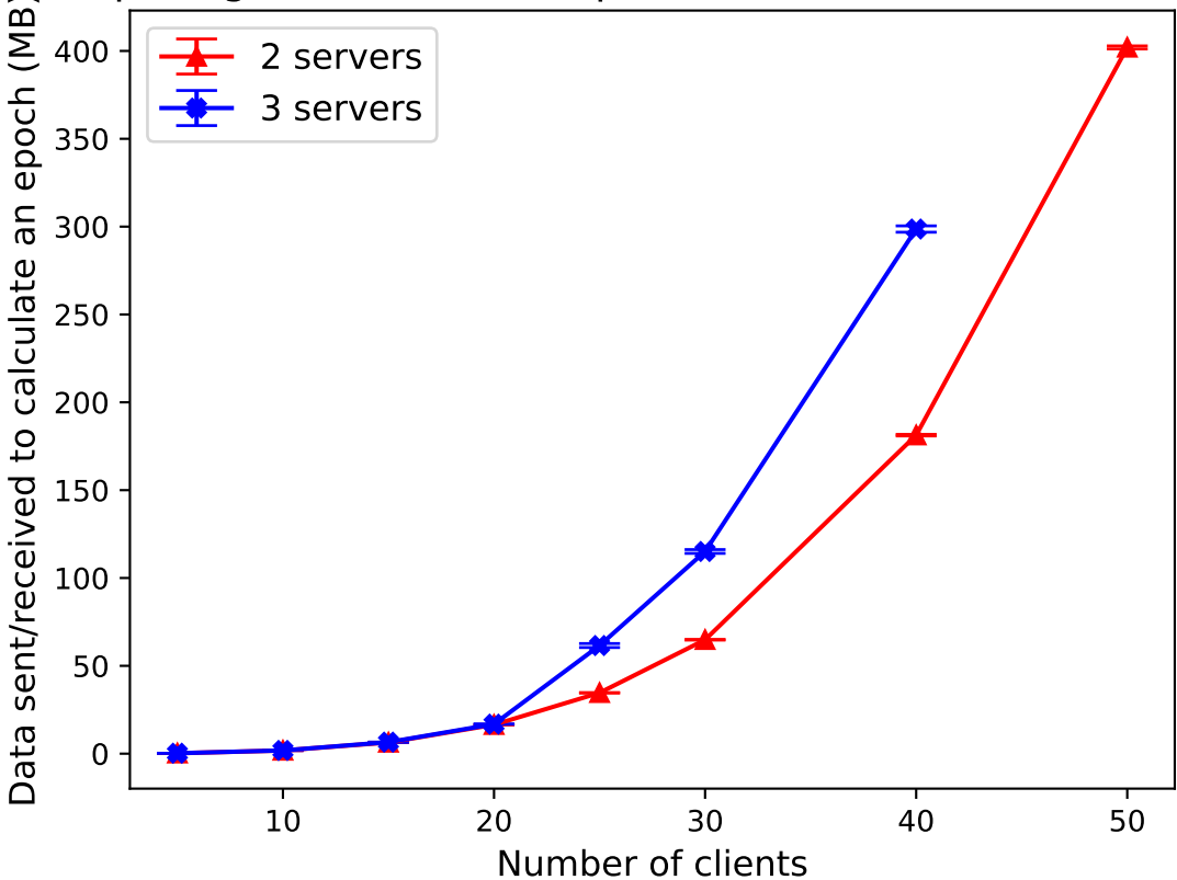
Comparing bandwidth for epochs across numbers of servers
