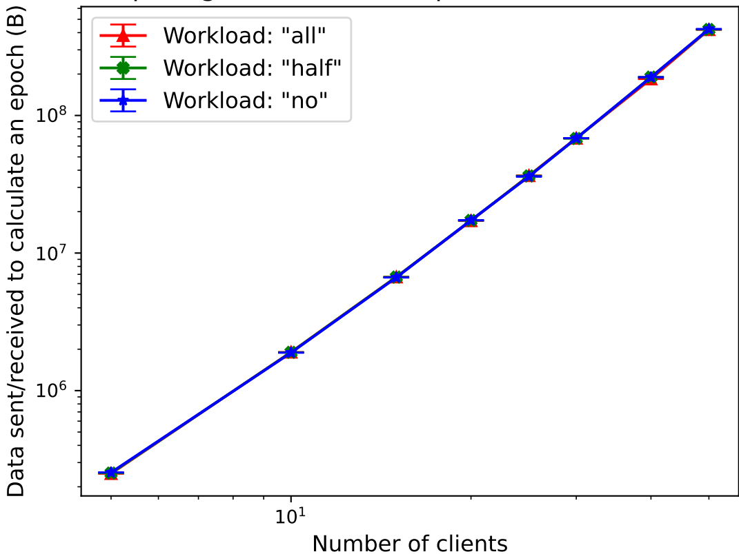
Comparing bandwidth for epochs across workloads
