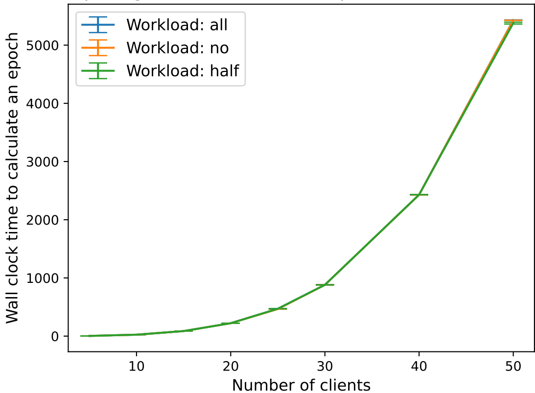
Comparing wall clock time for epochs across workloads
