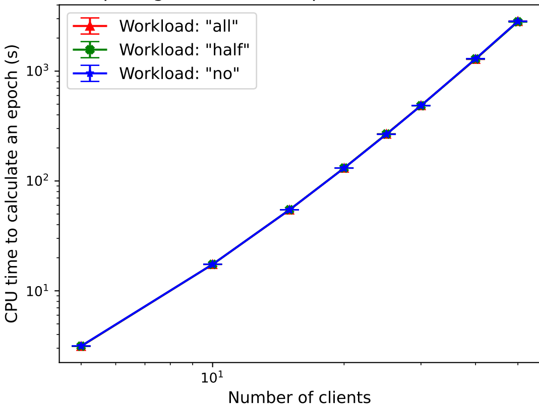
Comparing CPU time for epochs across workloads
