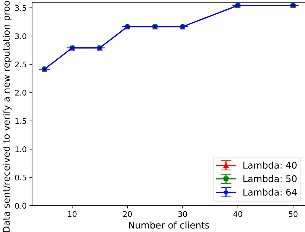
Comparing bandwidth for verifying reputation proofs across different values of lambda
