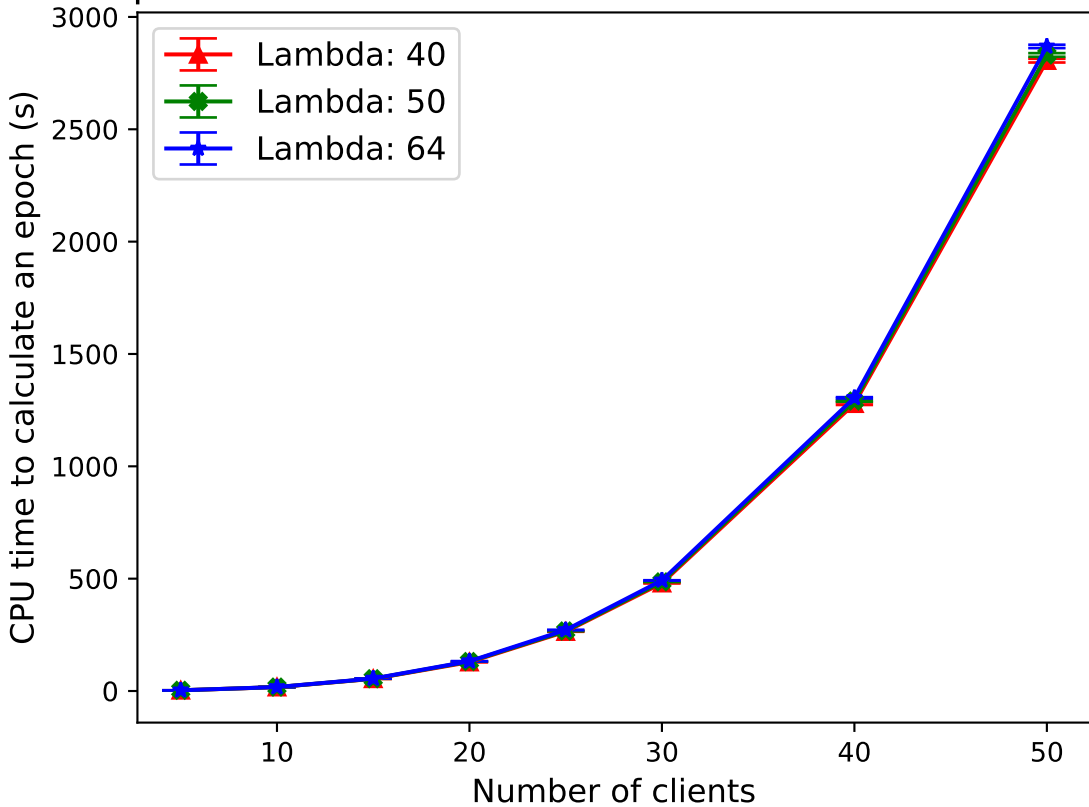
Comparing CPU time for covert security epoch calculations across different values of lambda
