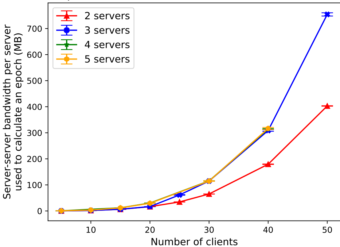
Comparing bandwidth for covert security epoch calculations across numbers of servers
