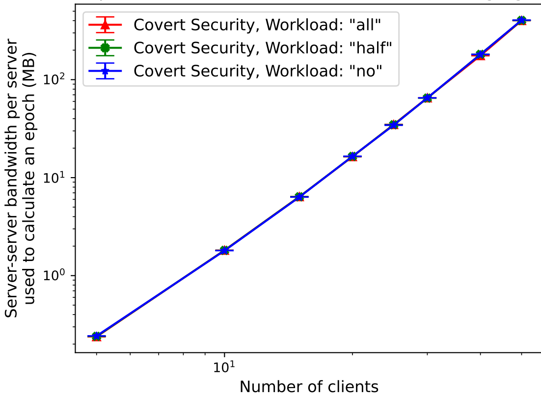
Comparing bandwidth for covert security epoch calculations across workloads (in loglog)
