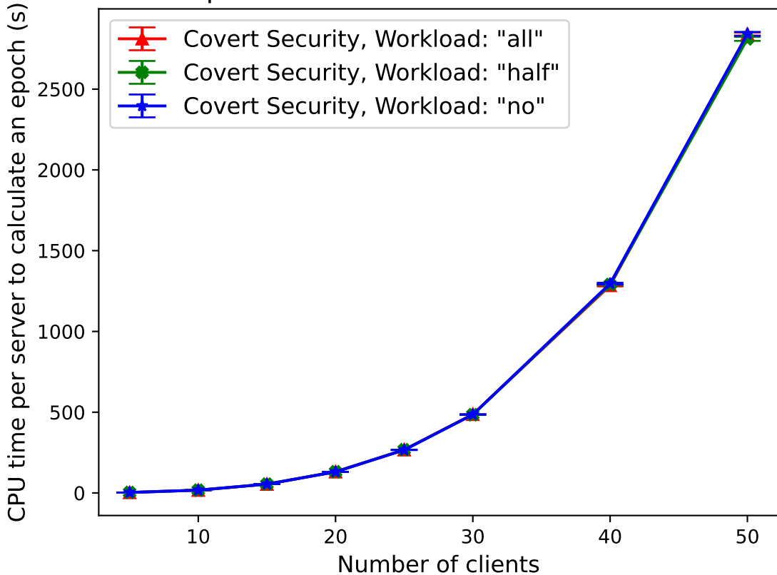
Comparing CPU time for covert security epoch calculations across workloads
