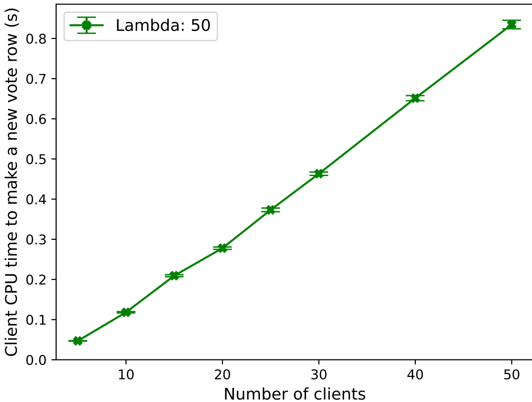
Measuring CPU time for making vote rows (in linear scale)
