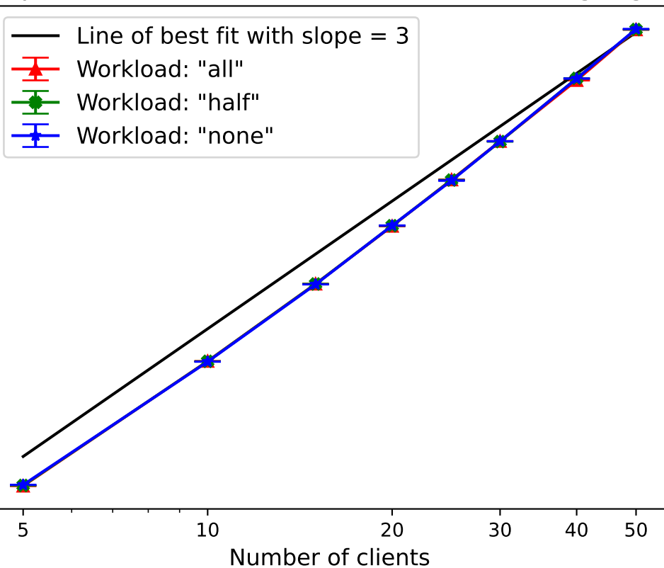
Comparing bandwidth for covert security epoch calculations across workloads (in log-log)
