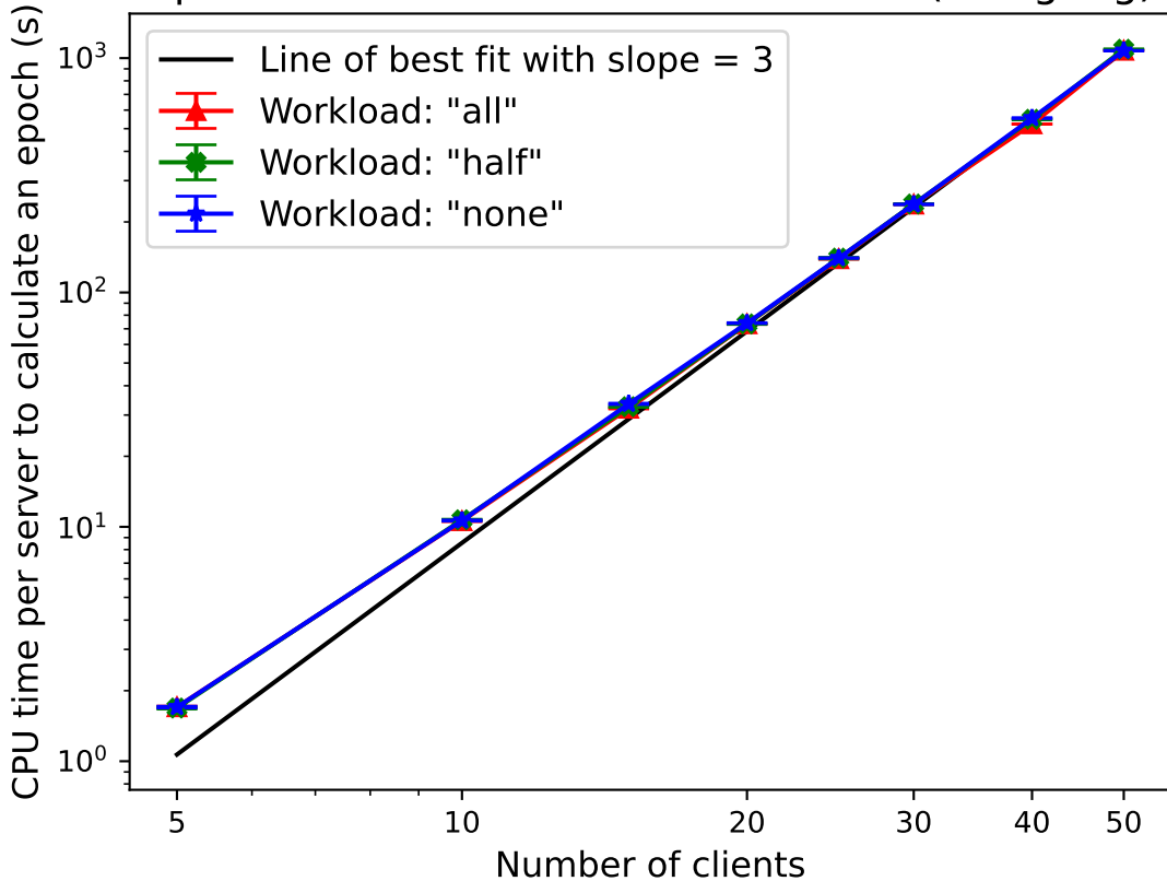
Comparing CPU time for HBC security epoch calculations across workloads (in log-log)
