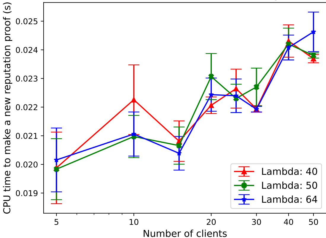
Comparing CPU time for making reputation proofs across different values of lambda (in log-linear)
