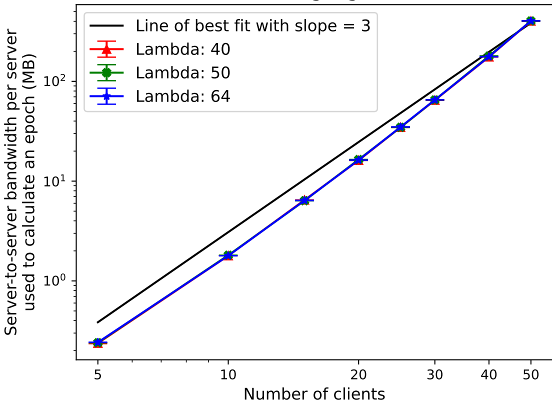
Comparing bandwidth for covert security epoch calculations across different values of lambda (in log-log)
