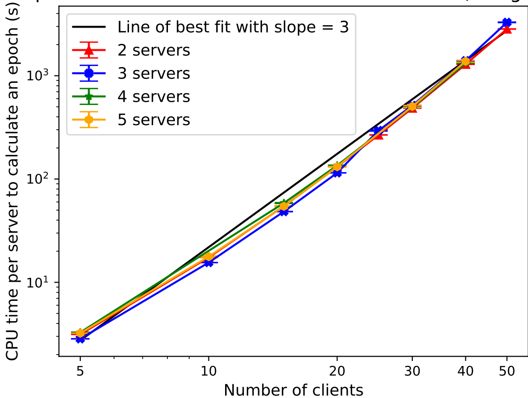
Comparing CPU time for covert security epoch calculations across numbers of servers (in log-log)
