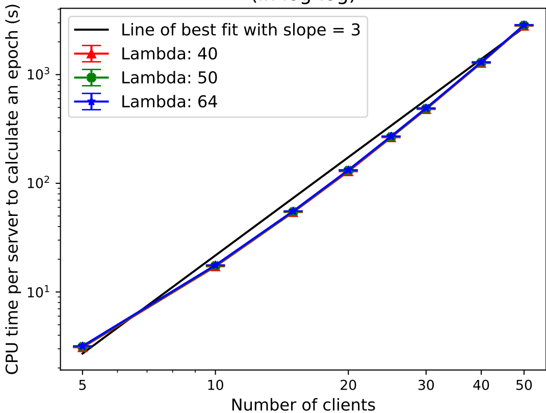
Comparing CPU time for covert security epoch calculations across different values of lambda (in log-log)
