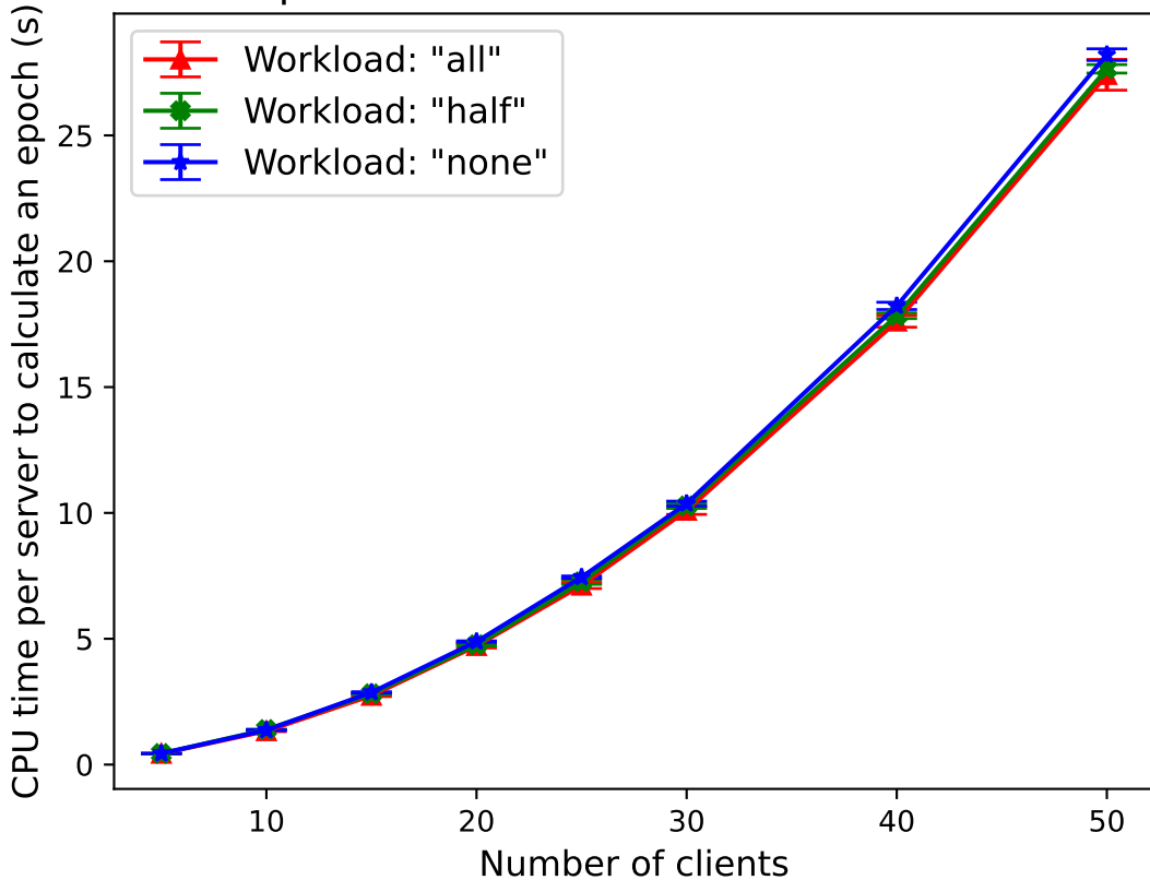
Comparing CPU time for HBC security epoch calculations across workloads
