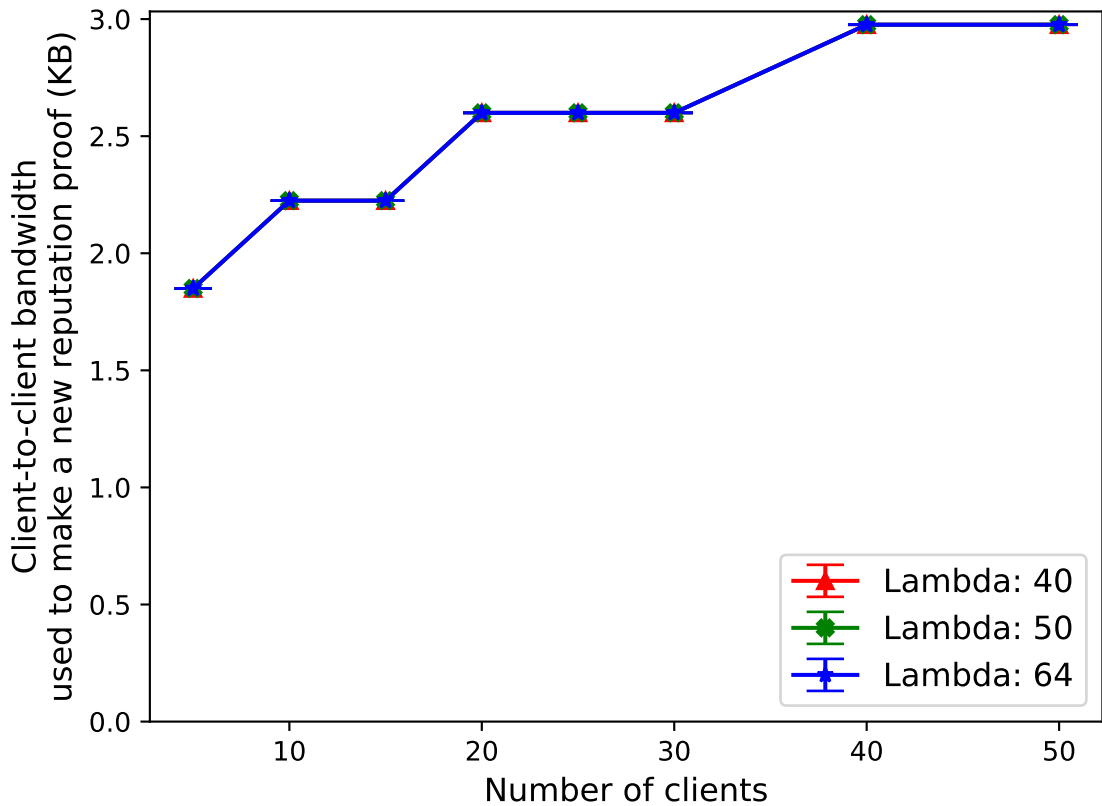
Comparing bandwidth for making reputation proofs across different values of lambda
