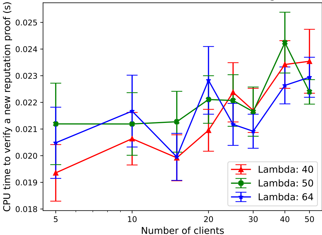
Comparing CPU time for verifying reputation proofs across different values of lambda (in log-linear)
