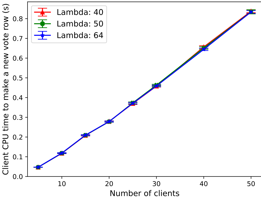
Comparing CPU time for making vote rows across different values of lambda (in linear scale)
