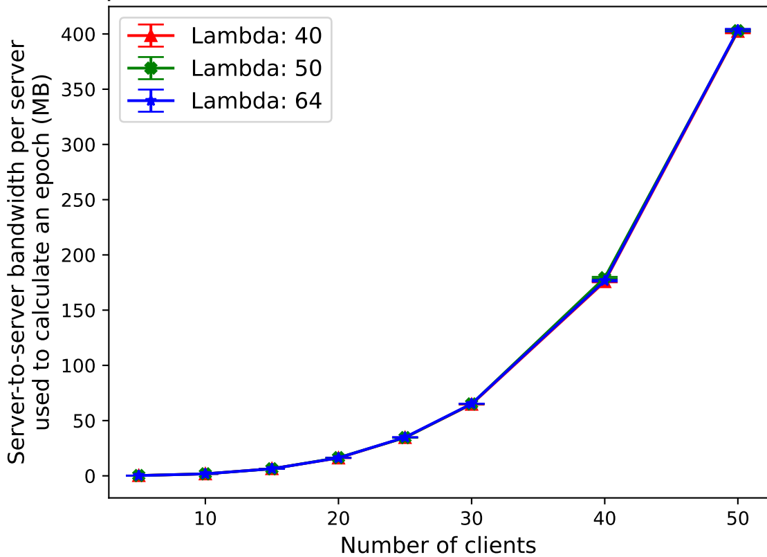
Comparing bandwidth for covert security epoch calculations across different values of lambda
