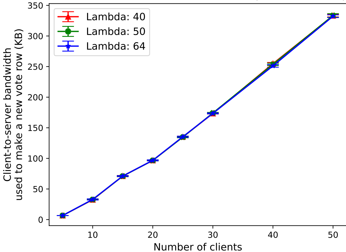
Comparing bandwidth for making vote rows across different values of lambda (in linear scale)
