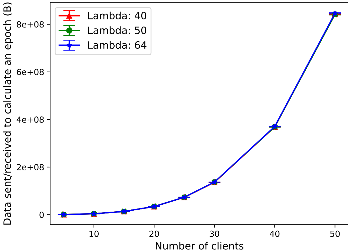
Comparing bandwidth for epochs across different values of lambda
