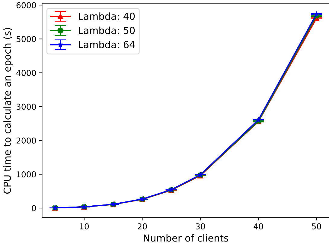
Comparing CPU time for epochs across different values of lambda
