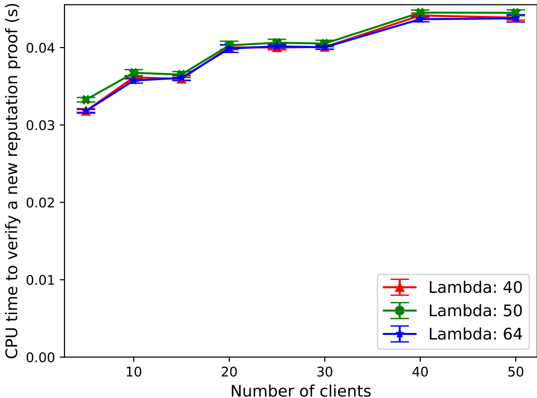
Comparing CPU time for verifying reputation proofs across different values of lambda
