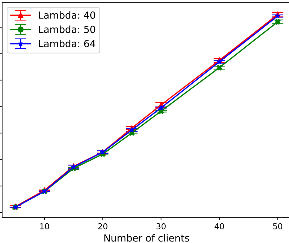
Comparing bandwidth for making vote rows across different values of lambda
